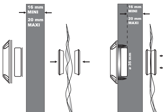
Drilling diameter: 35 mm, identical to the drilling diameter for a hinge
