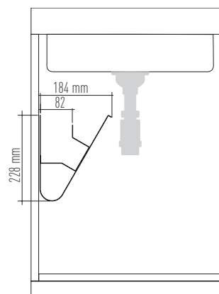
Under-sink unit front view
